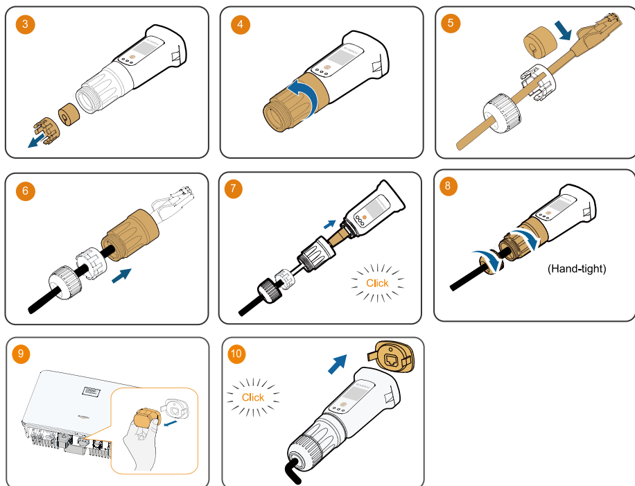
COM (Meter, RS485, CAN, DRM)
